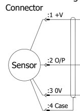
Connector
